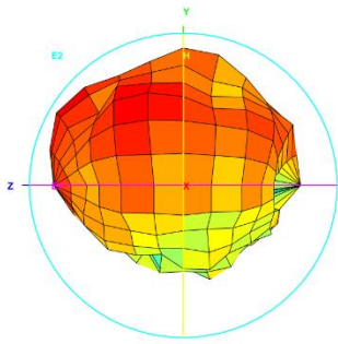
Total_3D_Top View_5.5GHz
